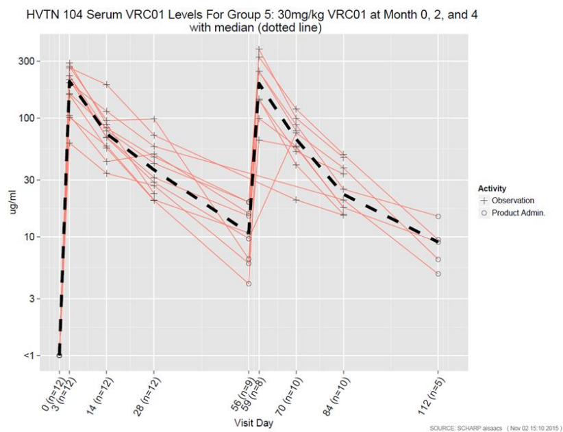
Figure 2-9 VRC01 serum levels through month 4 observed in HVTN 104 Group 4 (10mg/kg IV) and Group 5 (30mg/kg IV)
