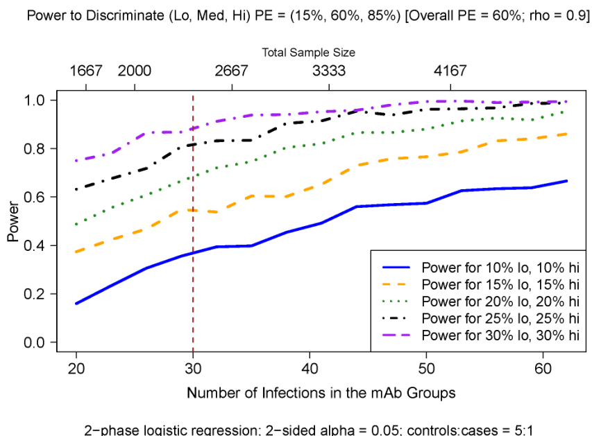
Figure 4-10 Power of the trial for detecting that PE varies over the three mAb marker-defined subgroups S(t) = Low, S(t) = Medium, and S(t) = High at level PE = 15%, 60%, 85%, respectively, for a marker with assay noise parameter \rho = 0.9 and percentages of person-years at risk in the Low and High marker regions varied from 10%, 15%, 20%, 25%, 30%. The calculations at 2700 total participants assume 30 mAb group HIV-1–infected cases and 150 mAb group HIV-1–uninfected controls with data on S(t) and pool over both mAb groups.
