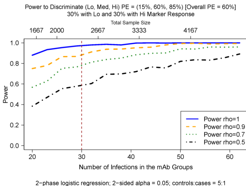
Figure 4-9 Power of the trial for detecting that PE varies over the three mAb marker-defined subgroups S(t) = Low, S(t) = Medium, and S(t) = High at level PE=15\% , 60\% , 85\% , respectively, for a marker with assay noise parameter \rho = 1 (perfect marker), 0.9 , 0.7 , and 0.5 and percentages of person-years at risk in the (Low, Medium, High) marker regions set at (30%, 40%, 30%). The calculations at 2700 total participants assume 30 mAb group HIV-1–
